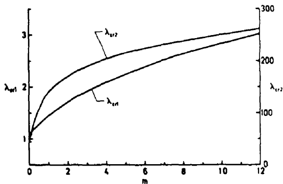
Fig. 2. Variation of the critical load factor \lambda_{cr} = P_{cr}(\rho_1 g h + p_0)/h with m = \mu_1(\kappa_2 + 1)/\mu_2(\kappa_1 + 1) . ( \lambda_{cr1} : tensile line load, \lambda_{cr2} : compressive line load).
